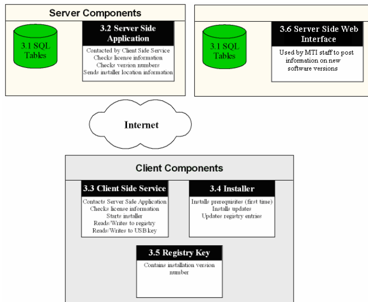
Fig 1. Components of the MTI's installer and update service
